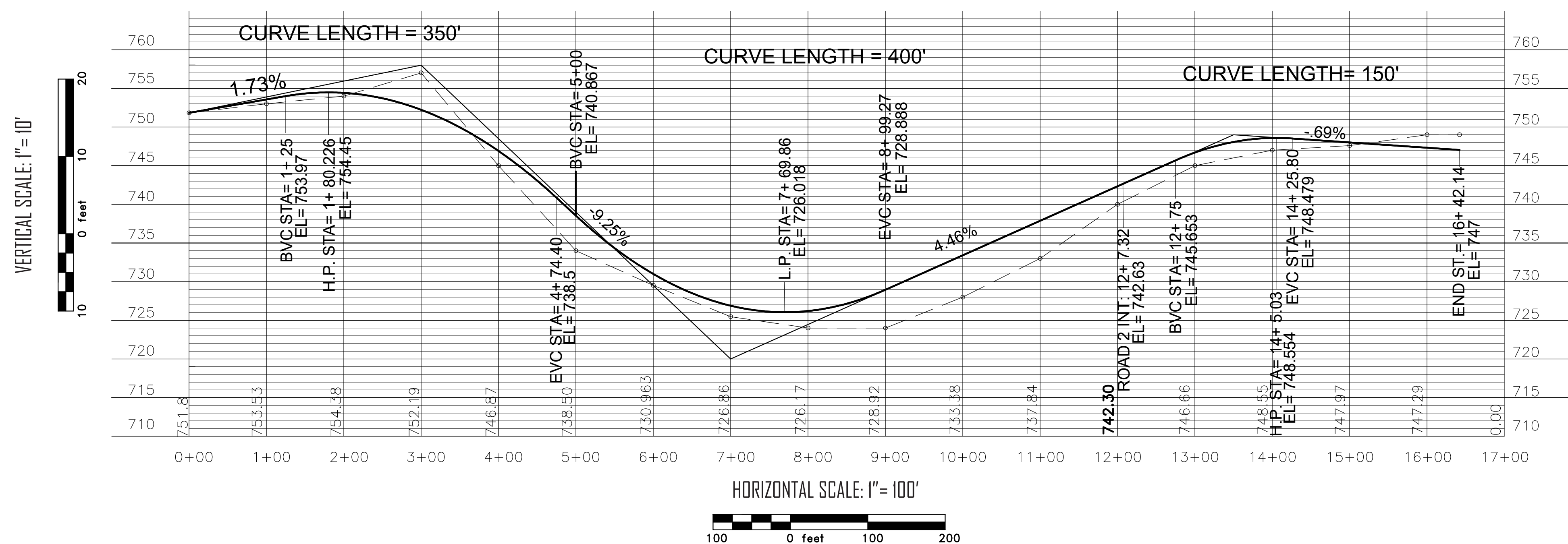
MINOR COLLECTOR ROAD VERTICAL PROFILE
