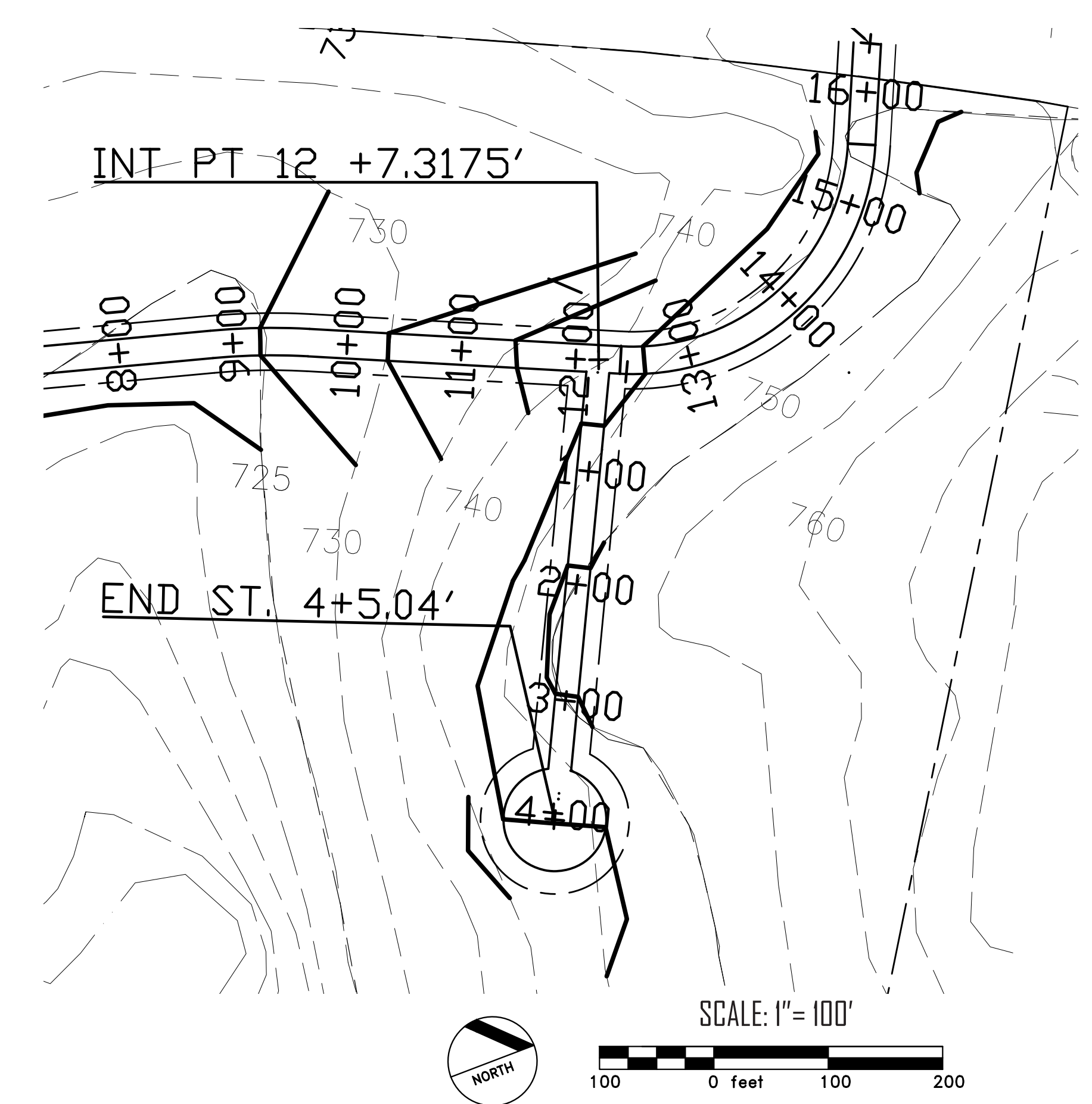
LOCAL ROAD GRADING PLAN
