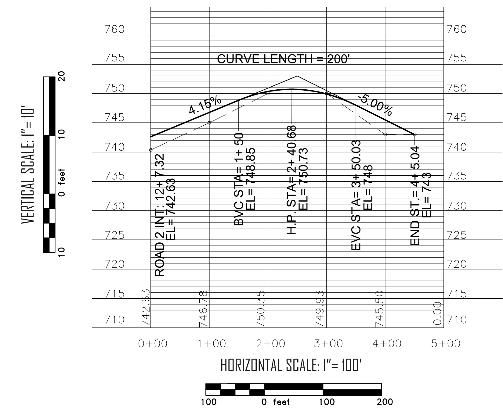
LOCAL ROAD VERTICAL PROFILE
