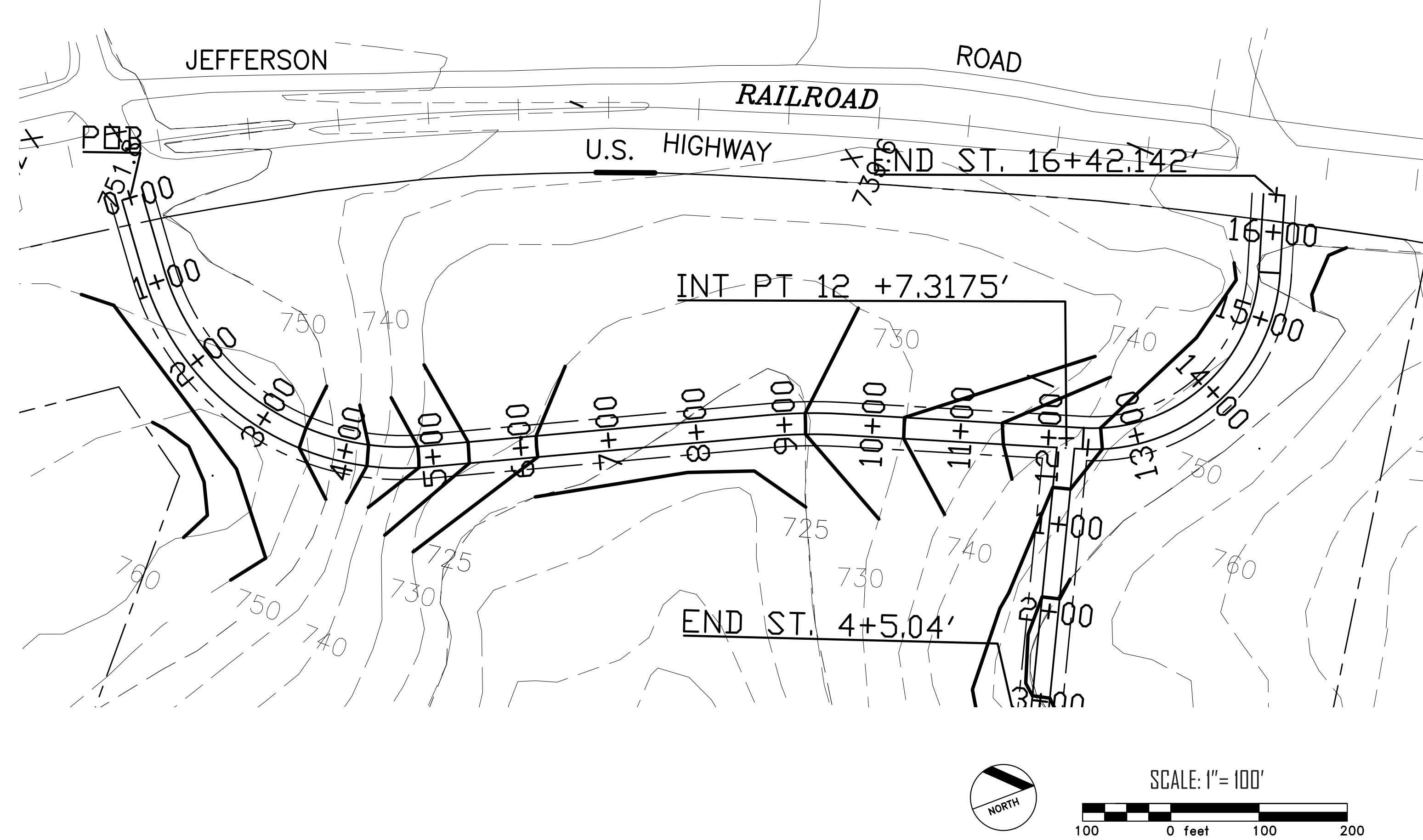
MINOR COLLECTOR ROAD GRADING PLAN
